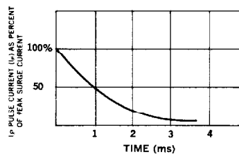
Pulse Waveform
